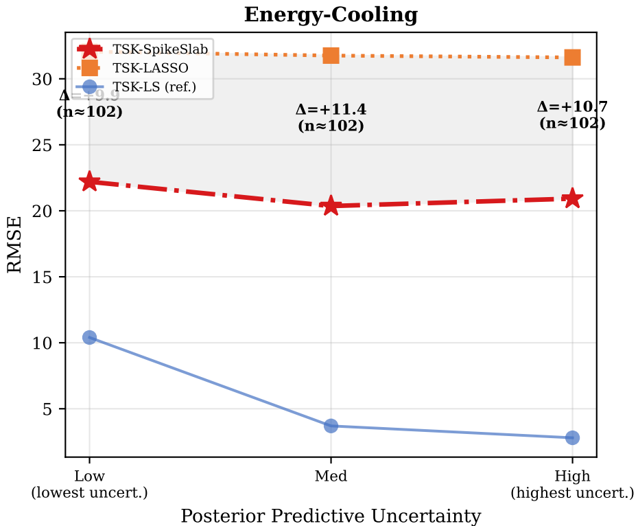
Fig. 3. Mechanism-probing: RMSE by uncertainty bin
