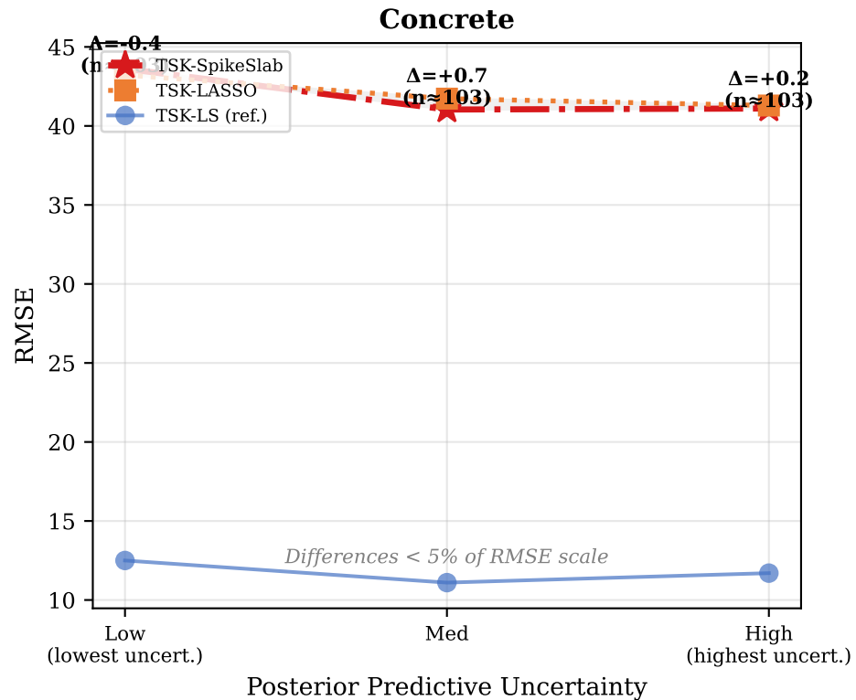
Fig. 3. Mechanism-probing: RMSE by uncertainty bin
