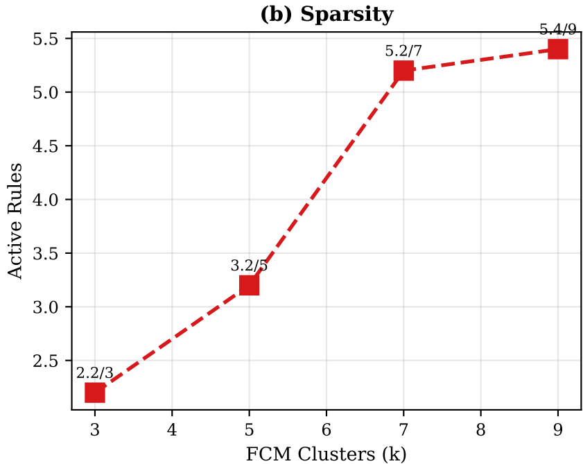
Fig. 4. Effect of FCM cluster count on accuracy and sparsity
