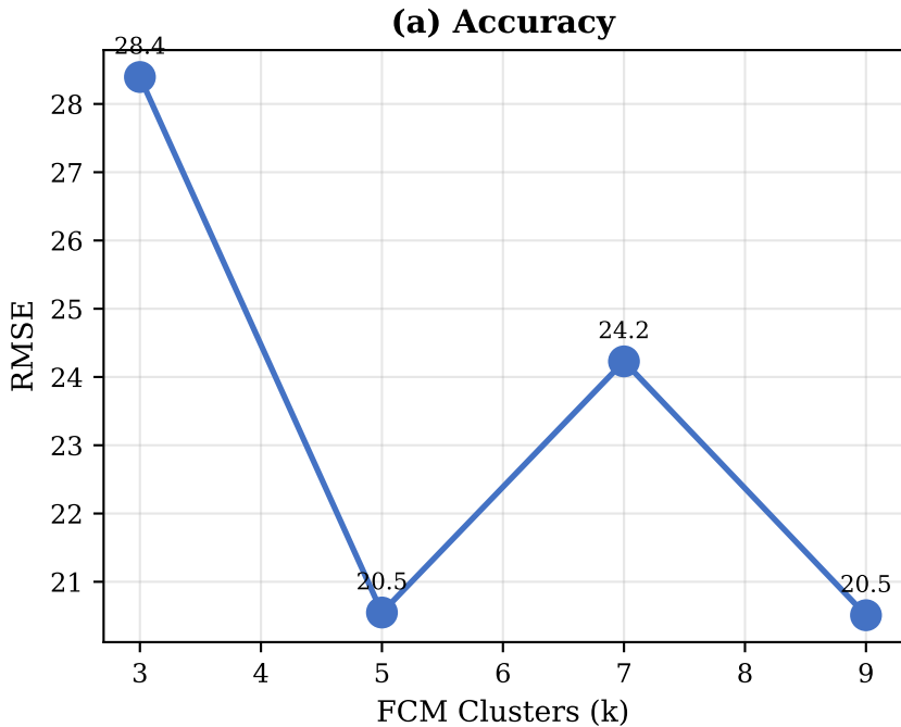
Fig. 4. Effect of FCM cluster count on accuracy and sparsity
