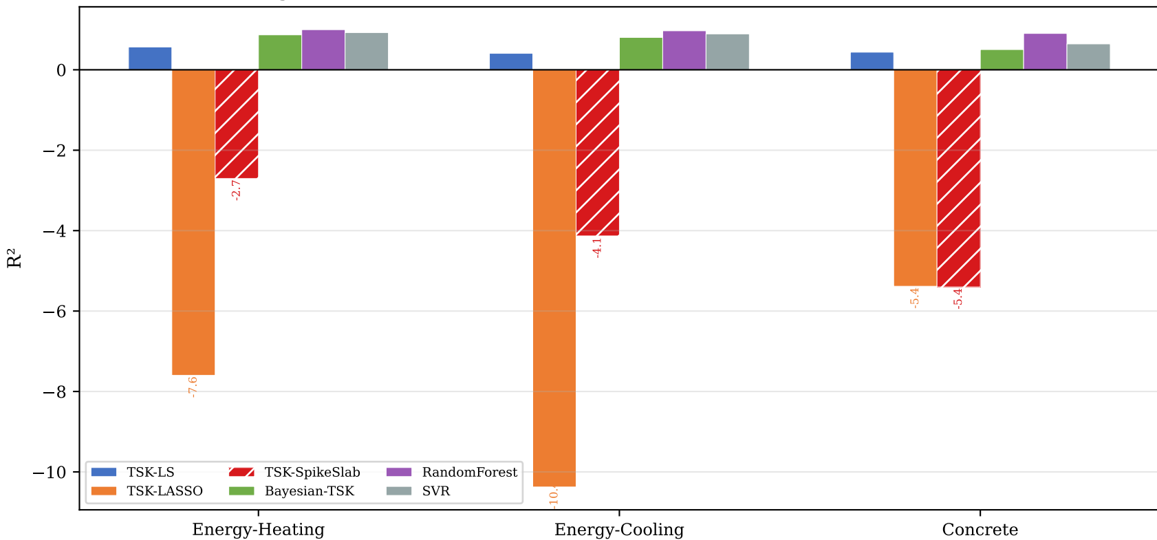
Fig. 7. Predictive performance ( R^2 ) across methods and datasets
