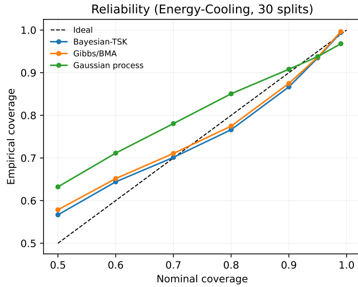
Figure 4: Empirical coverage versus nominal coverage for the conjugate Bayesian-TSK, the Gibbs/BMA sampler, and the Gaussian-process reference on Energy-Cooling (30 splits). Points on the diagonal would indicate perfectly calibrated intervals. The Bayesian methods over-cover at the lowest nominal levels (empirical coverage 0.57 at nominal 0.5). They under-cover slightly in the range 0.8–0.95 (empirical 0.94 at nominal 0.95) and return to the diagonal at nominal 0.99. The Gaussian process falls below the diagonal at nominal 0.99.
