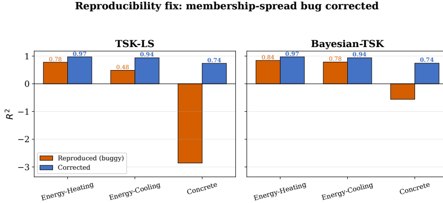
Figure 1: Corrected dense baselines. Reproduced R^2 under the buggy membership implementation (orange) versus corrected R^2 (blue, training-time membership spreads reused at inference) for the dense TSK-LS and conjugate Bayesian-TSK baselines. Values are means over 30 splits on the Energy (Heating and Cooling) and Concrete targets; correcting the membership-spread bug raises the dense TSK-LS R^2 from 0.48 to 0.94 on Energy-Cooling.
