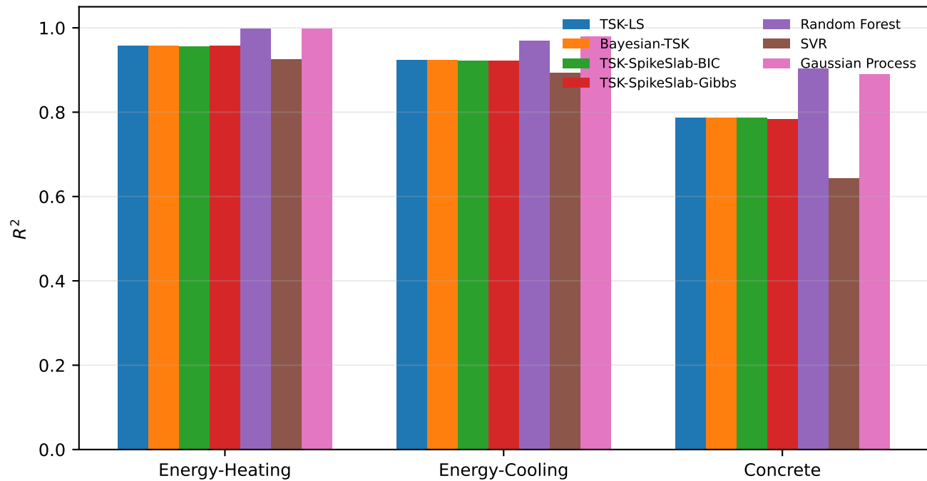
Predictive accuracy under the rebuilt protocol
