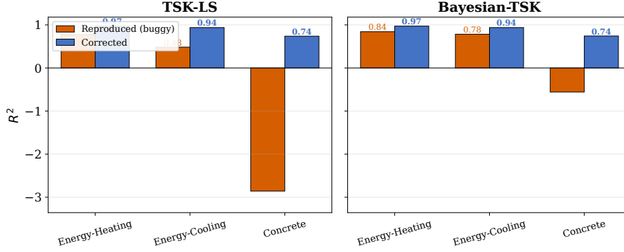
Figure 1: Corrected dense baselines. Reproduced R^2 under the buggy membership implementation (orange) versus corrected R^2 (blue, training-time membership spreads reused at inference) for the dense TSK-LS and conjugate Bayesian-TSK baselines. Values are means over 30 splits on the Energy (Heating and Cooling) and Concrete targets; correcting the membership-spread bug raises the dense TSK-LS R^2 from 0.48 to 0.94 on Energy-Cooling.
