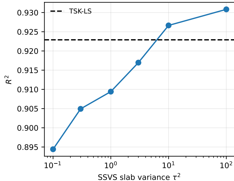
Coefficient-level sensitivity
