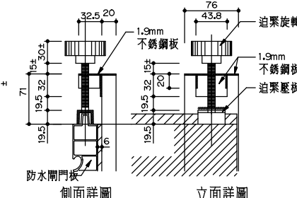
詳圖I UNIT=mm 12
