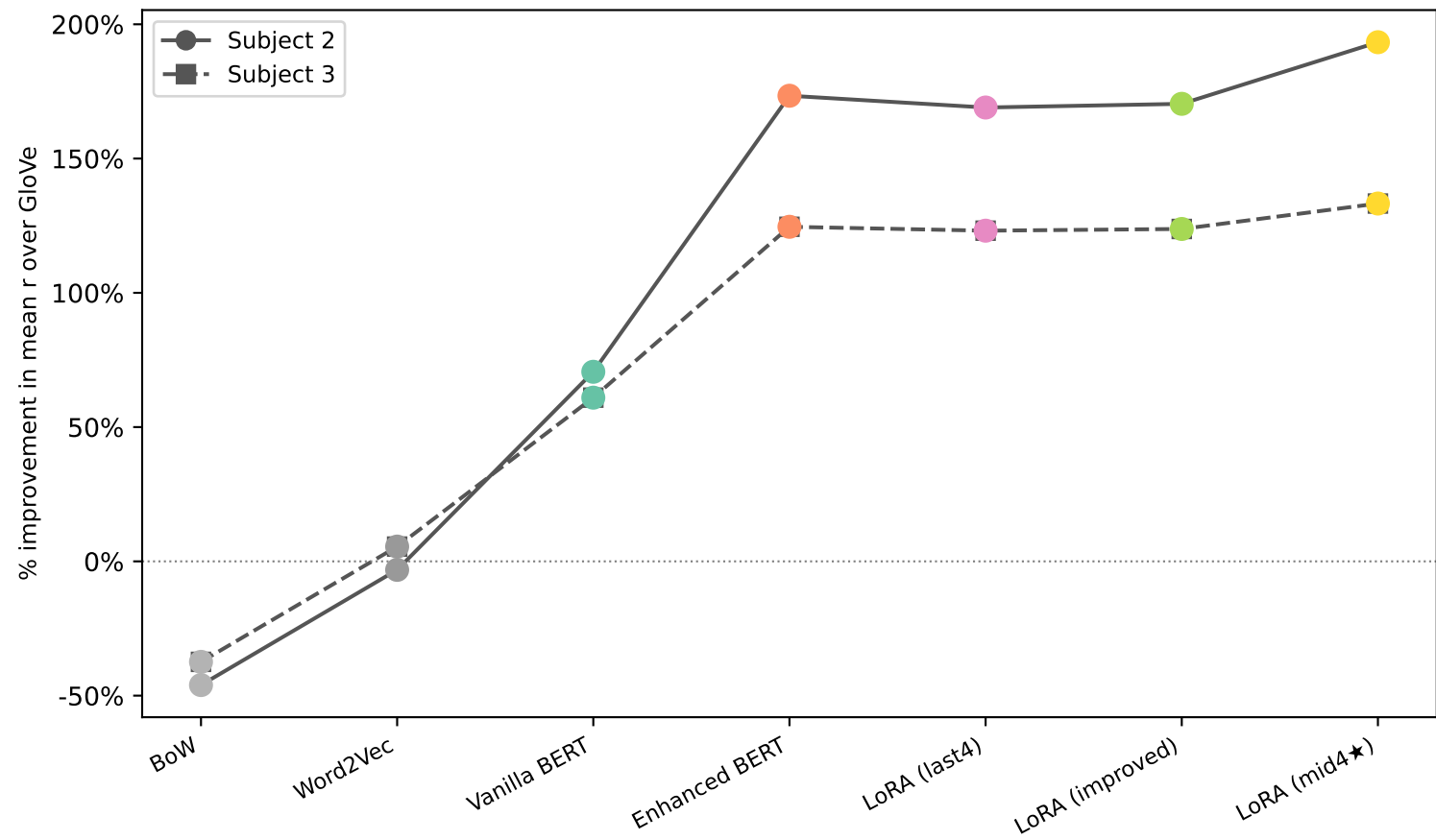
Relative Gain over GloVe Baseline
