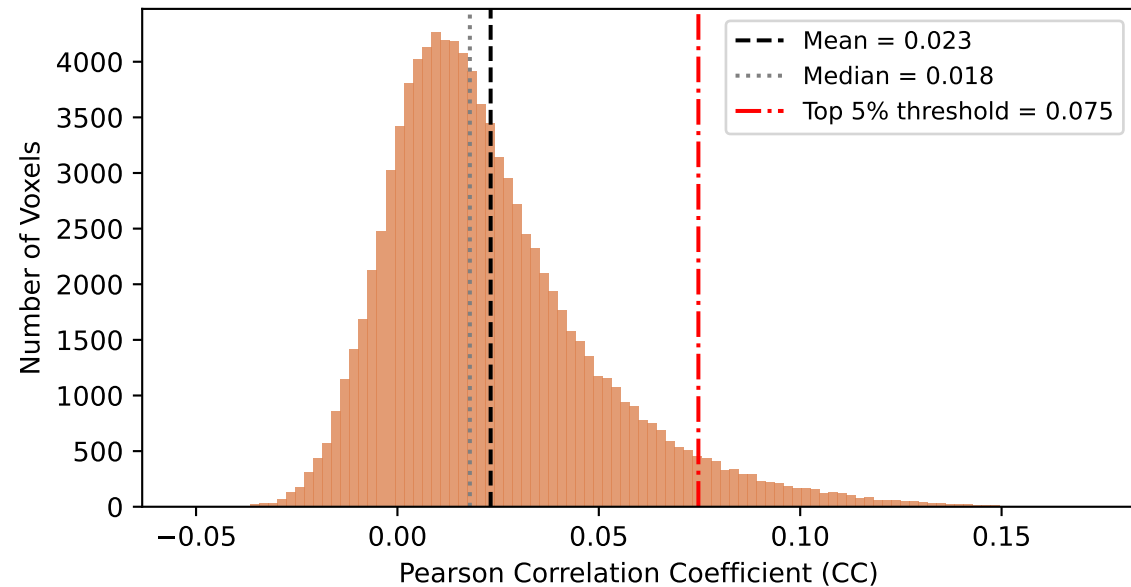
CC Distribution — Word2Vec, Subject 3 (all 95,556 voxels)
