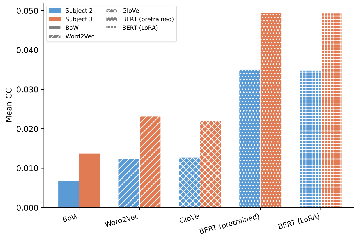
Mean CC
