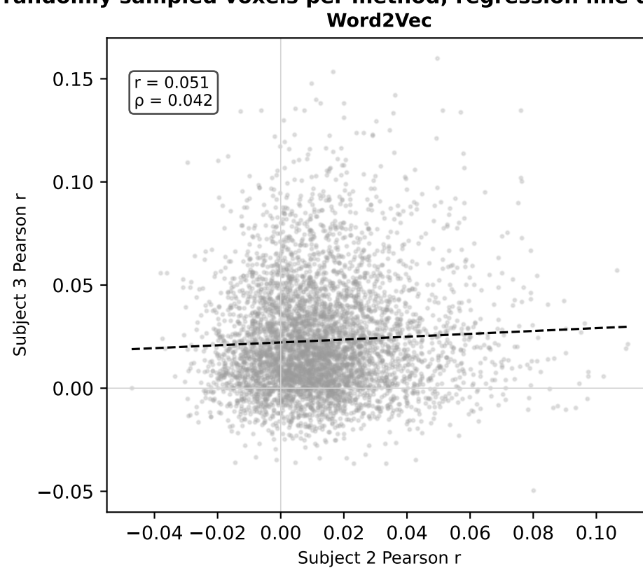
Cross-Subject Consistency: Per-voxel CC, Subject 2 vs Subject 3 (5 000 randomly sampled voxels per method; regression line dashed)
