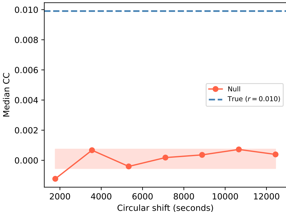
Median CC vs. Temporal Misalignment
