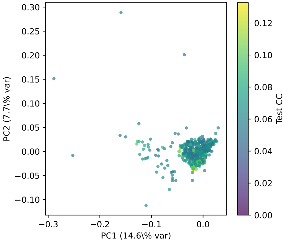
s2: Top-5\% Voxels — Functional PCA
