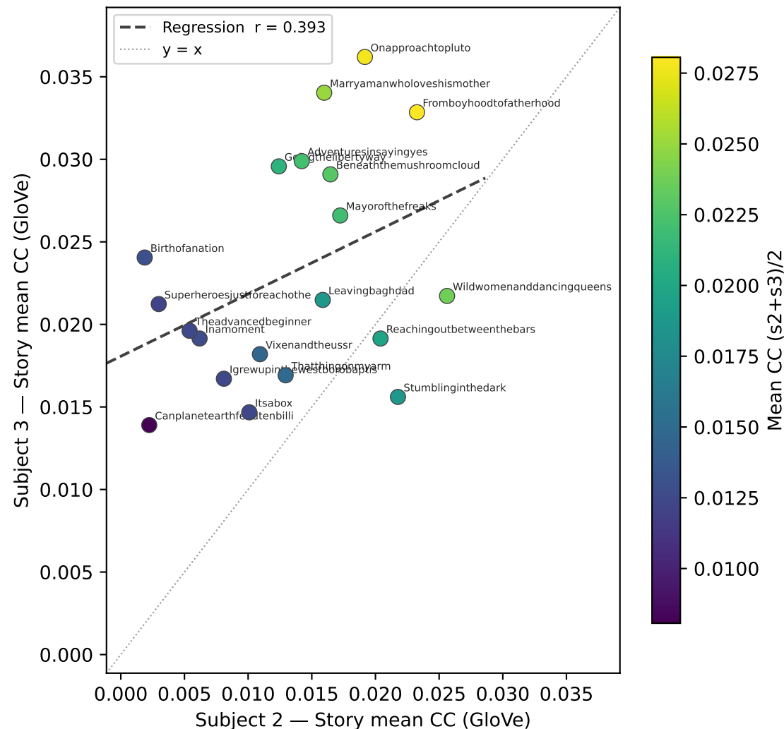
(A) Story-level Encoding Agreement Pearson r = 0.393 , n = 20 test stories
