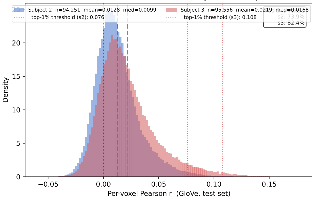
(C) Voxelwise CC Distributions — Subject 2 vs. Subject 3
