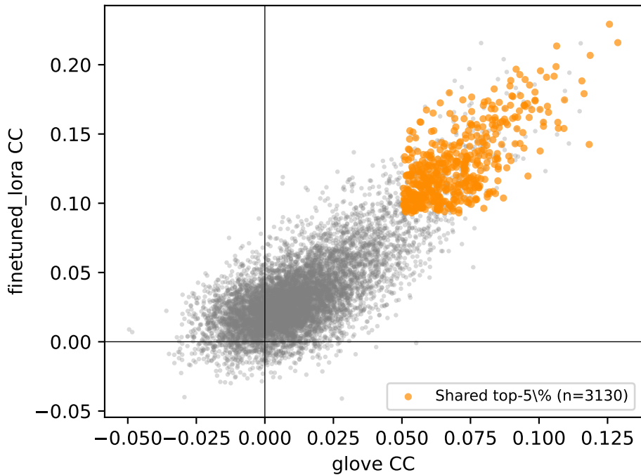
glove vs. finetuned_lora ( r = 0.745 )
