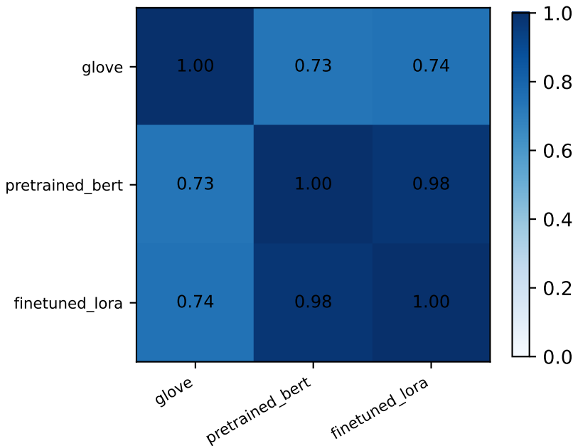
CC Profile Pearson r (per-voxel)
