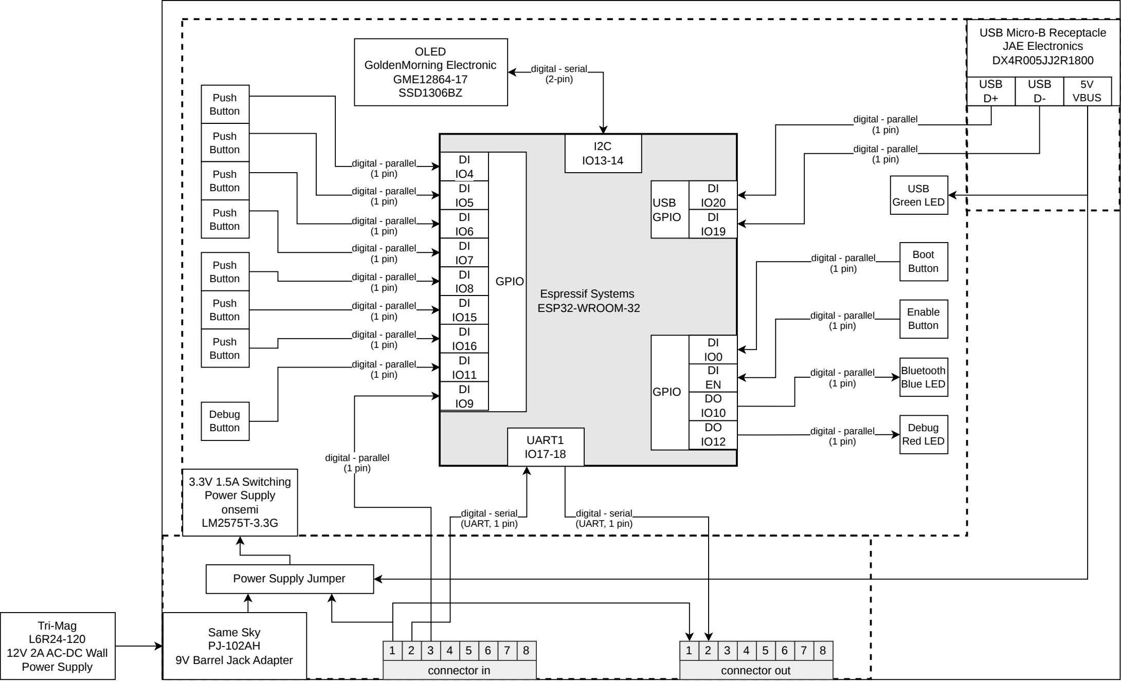
Block Diagram -- Jacob Alger Team 202 -- Exploration Device Project
