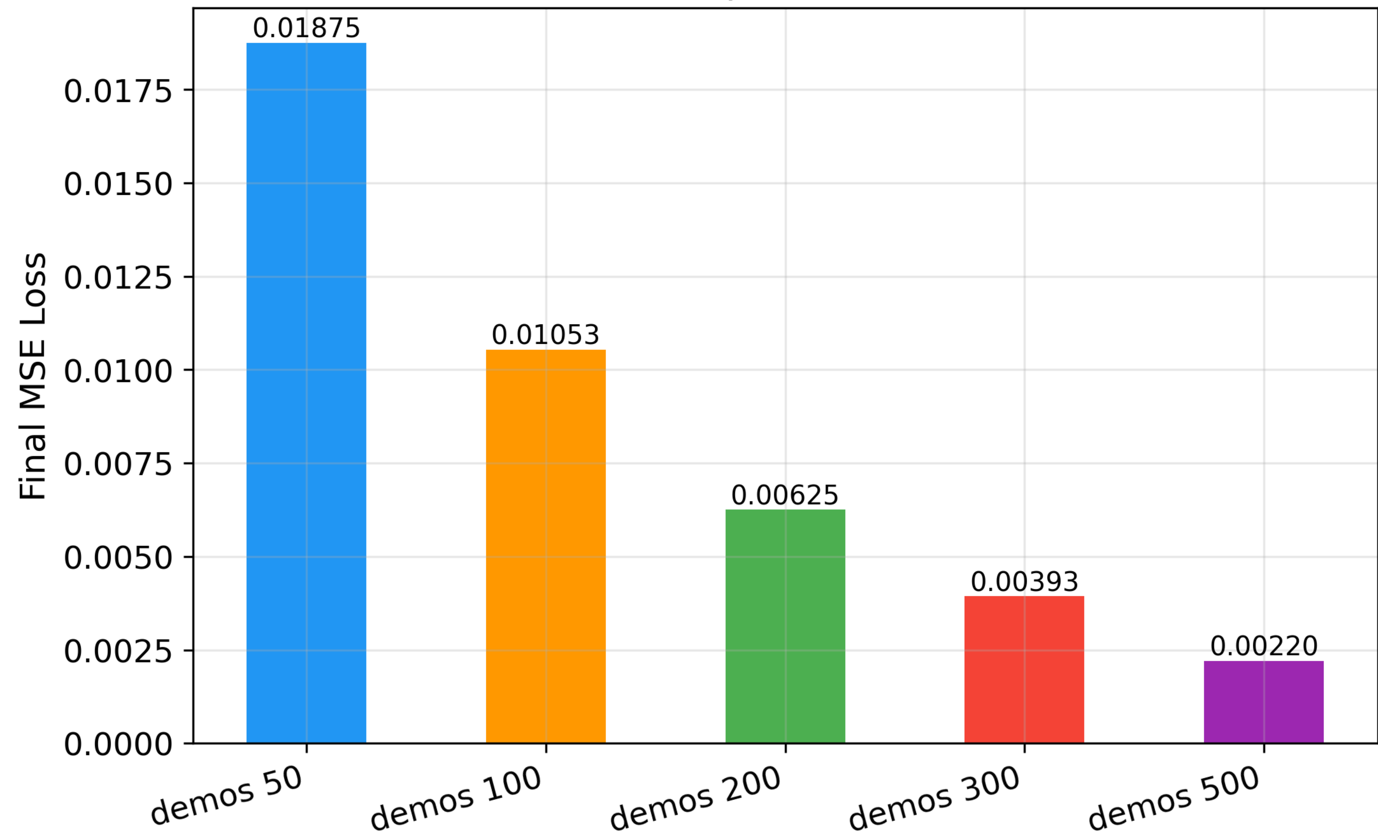
Final Loss Comparison: Demo Count
