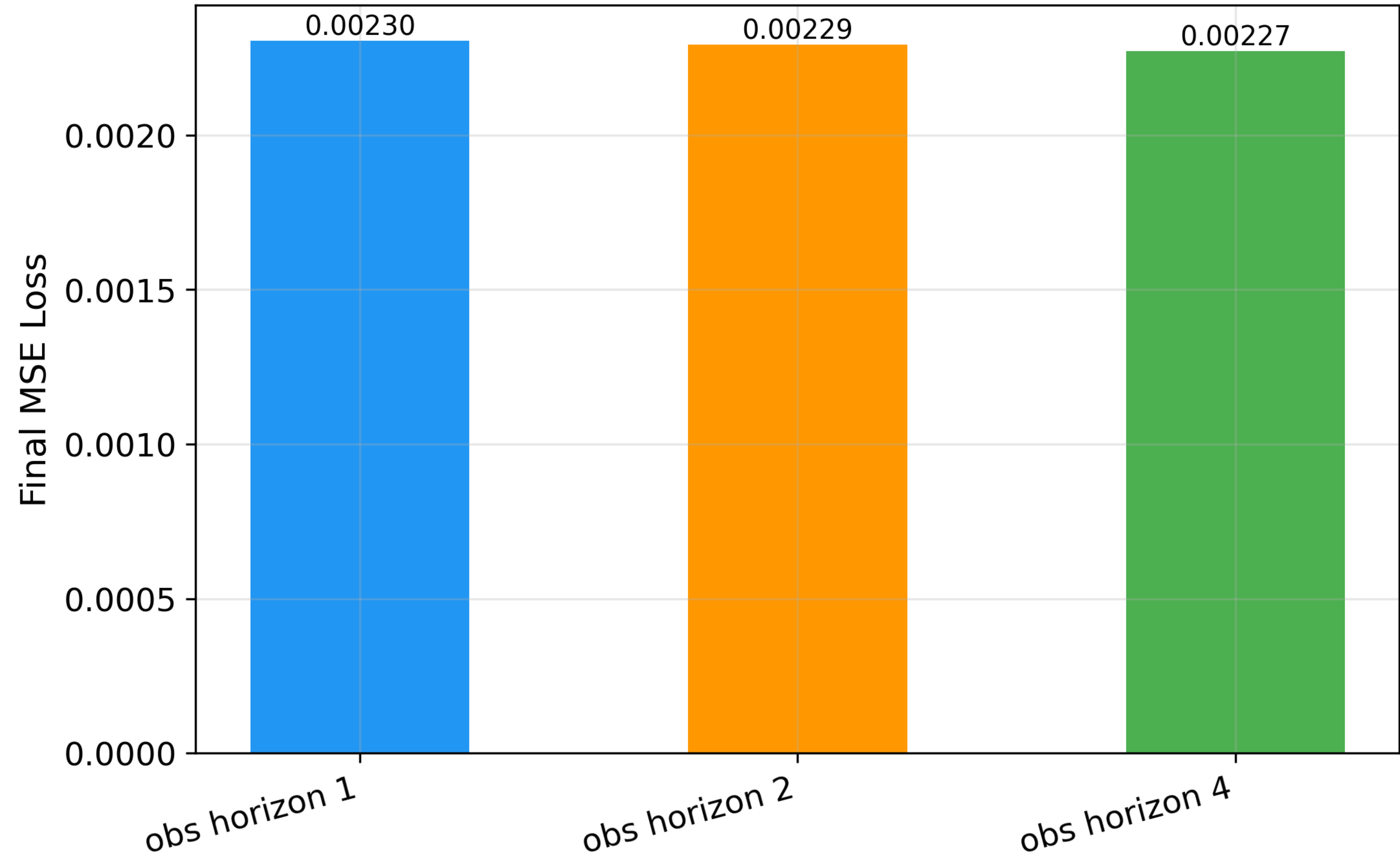
Final Loss Comparison: Observation Horizon
