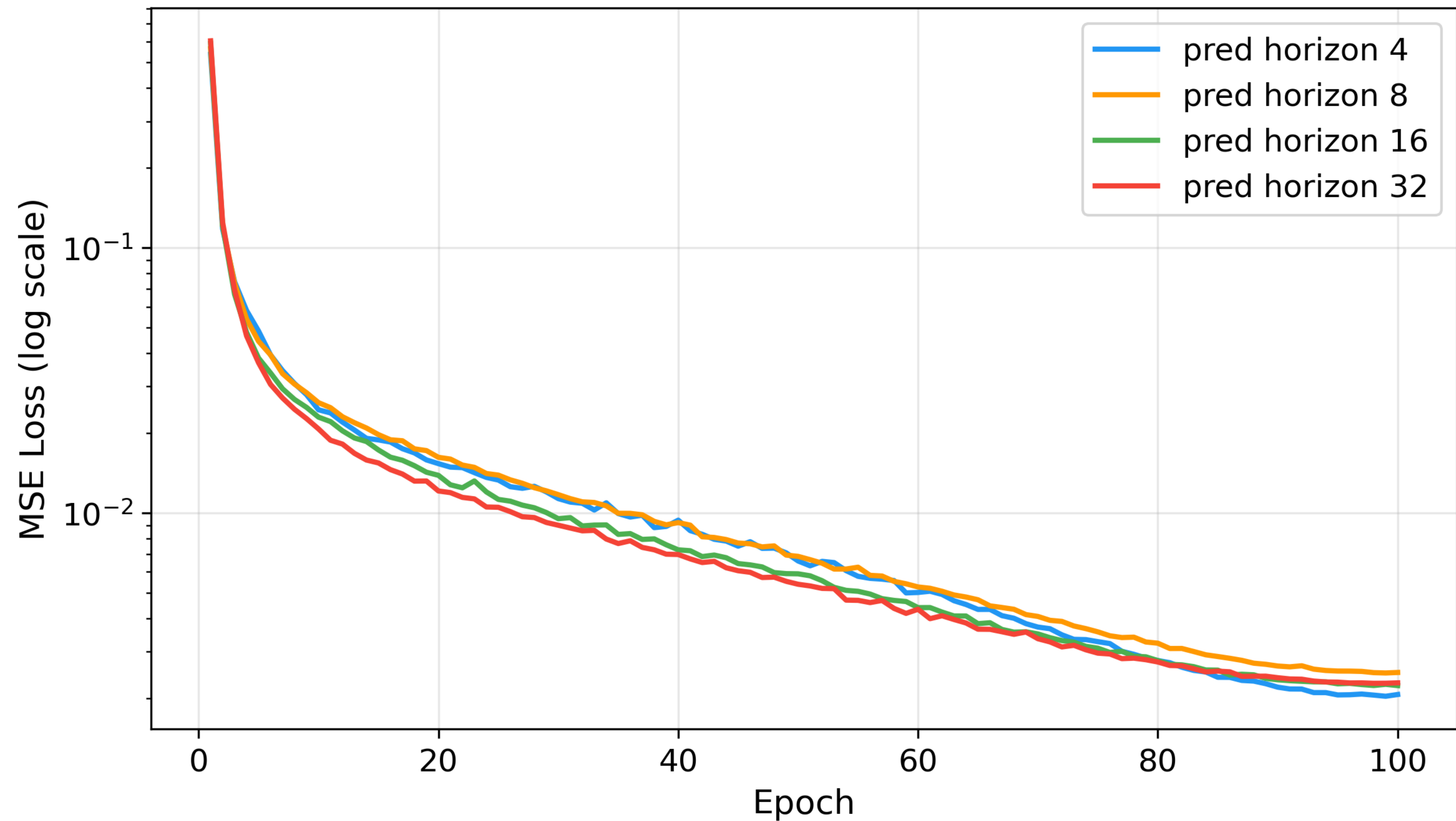
Ablation: Prediction Horizon
