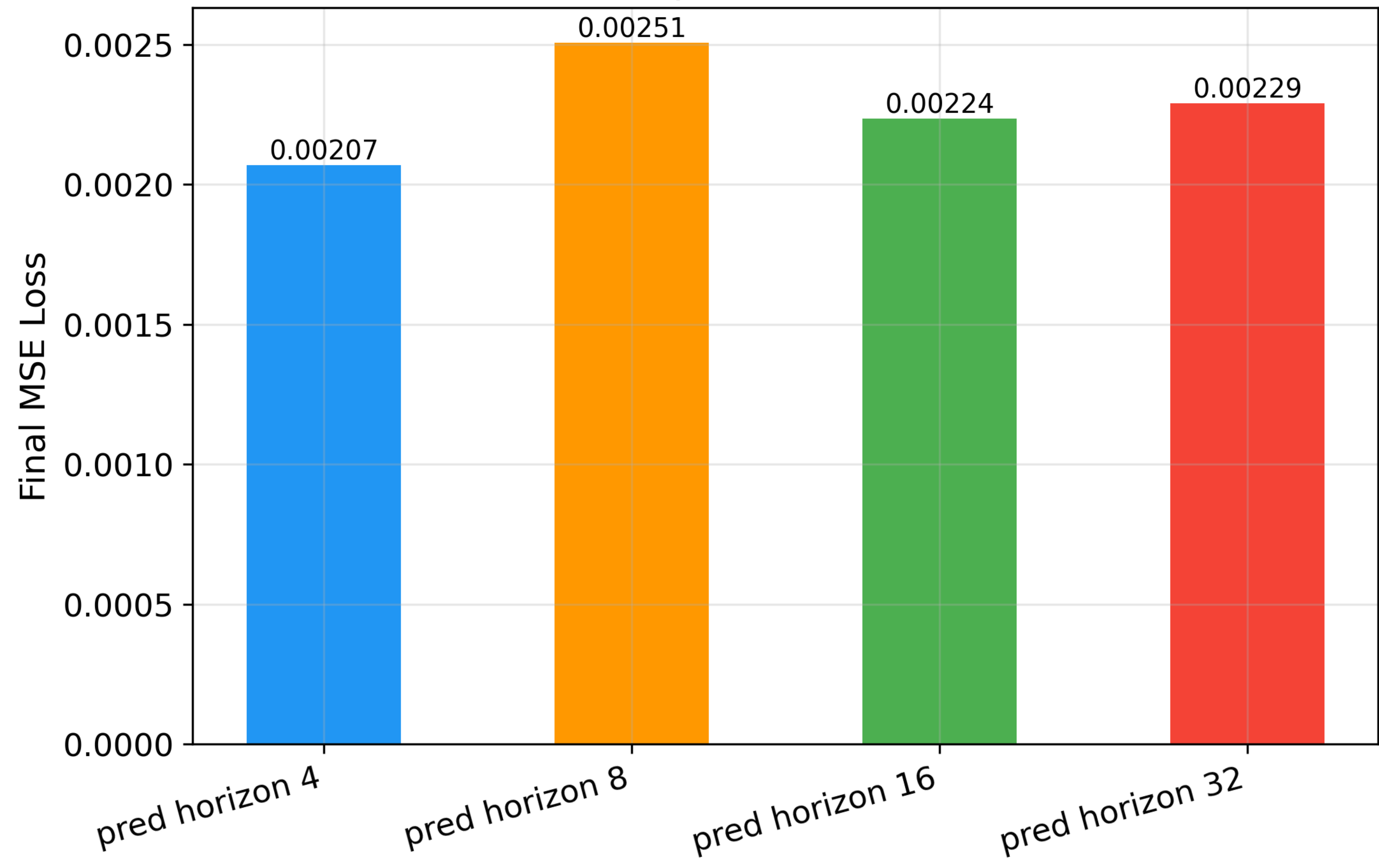
Final Loss Comparison: Prediction Horizon
