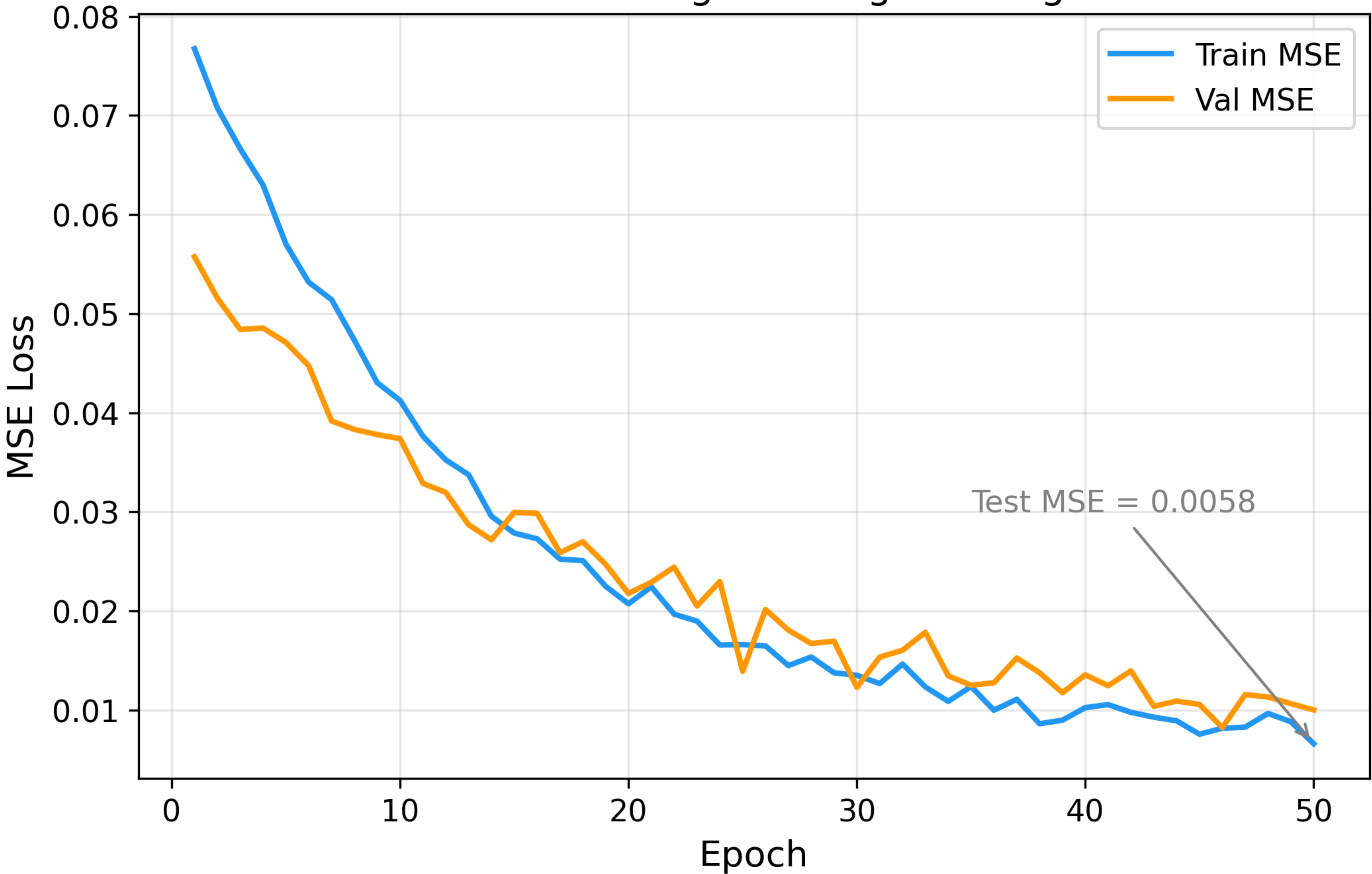
Behavioral Cloning: Training Convergence
