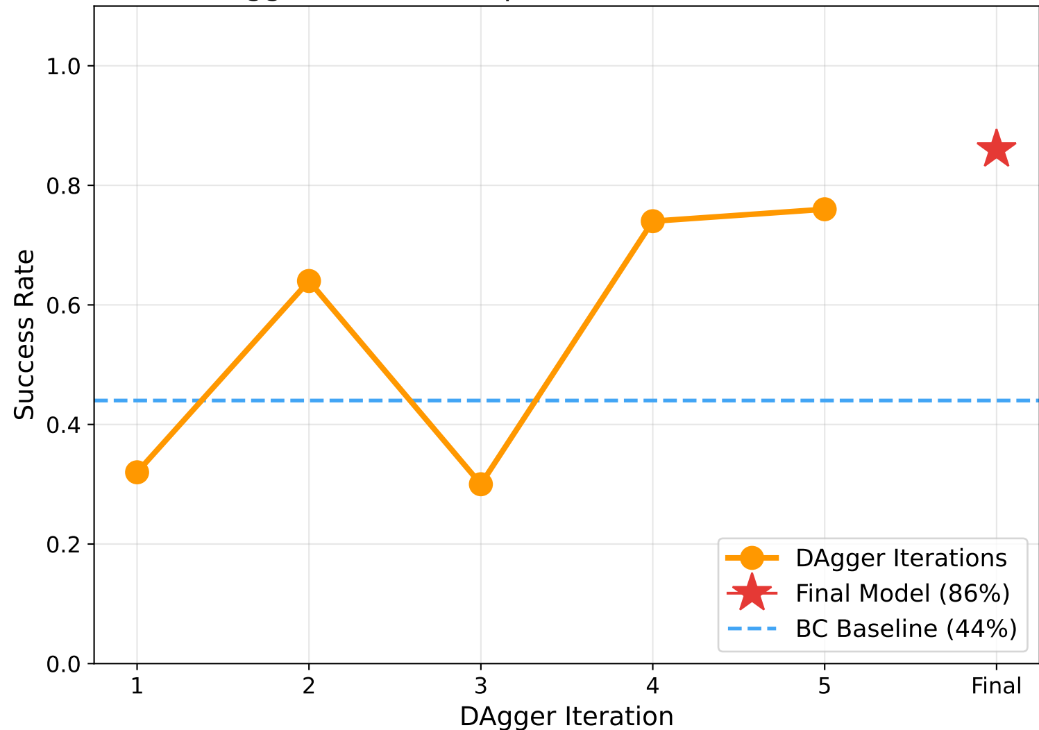
DAgger: Iterative Improvement Over BC Baseline
