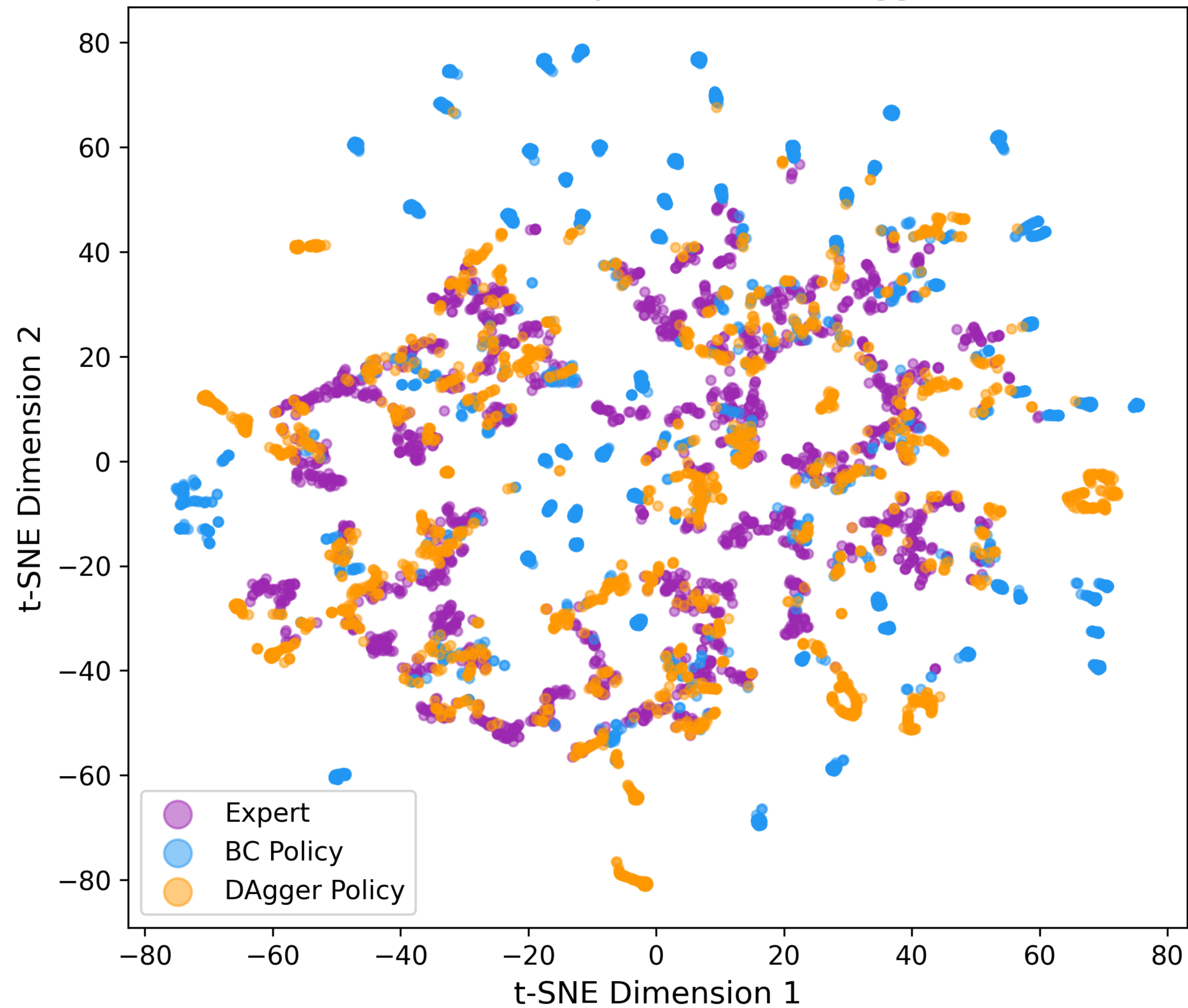
State Distribution: Expert vs BC vs DAgger (t-SNE)
