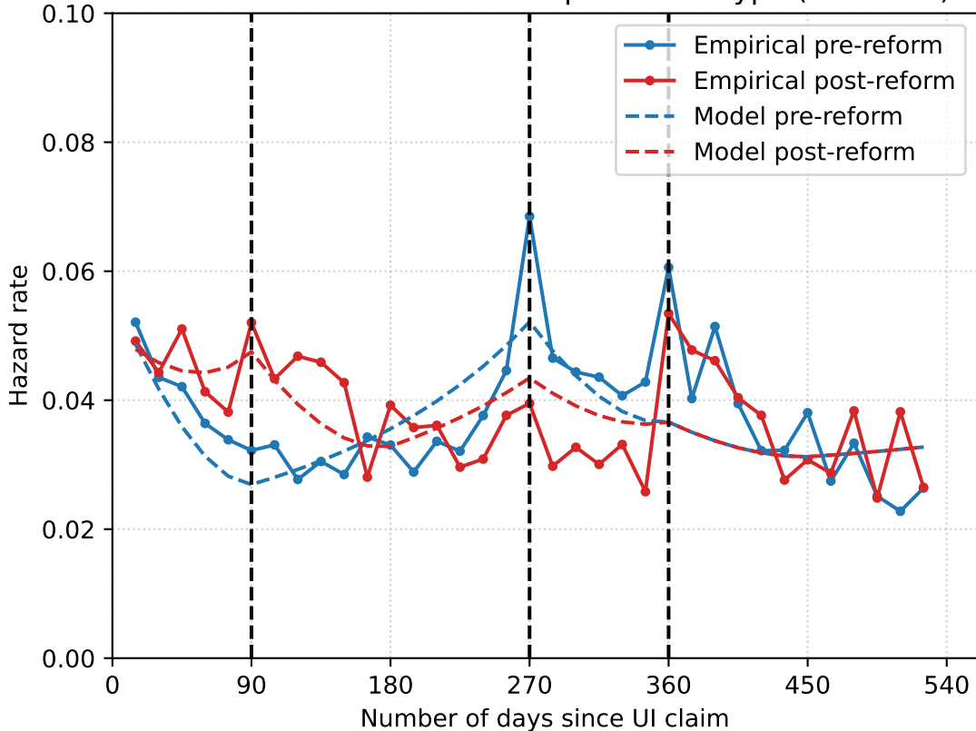
Estimated fit — Reference dependent 1 type (L-BFGS-B)
