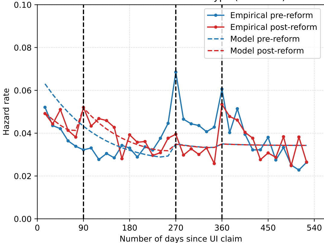
Estimated fit — Standard 2 type (L-BFGS-B)
