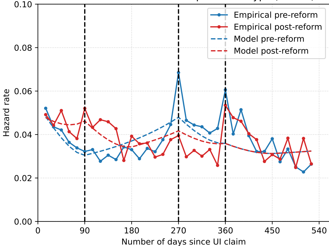
Estimated fit — Reference dependent 1 type (LS-TRF)
