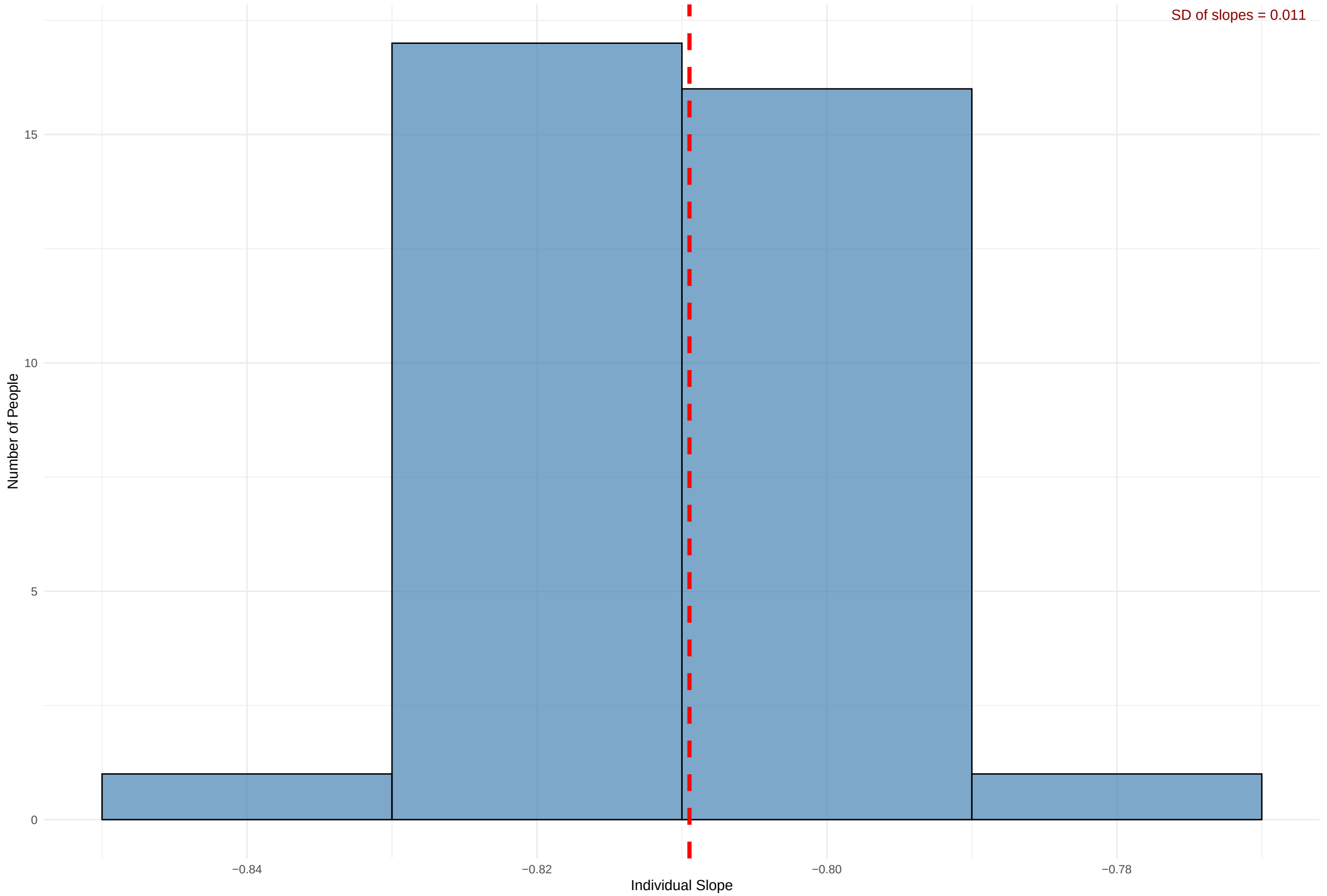
Distribution of Individual Slopes (Activity -> Mood)
