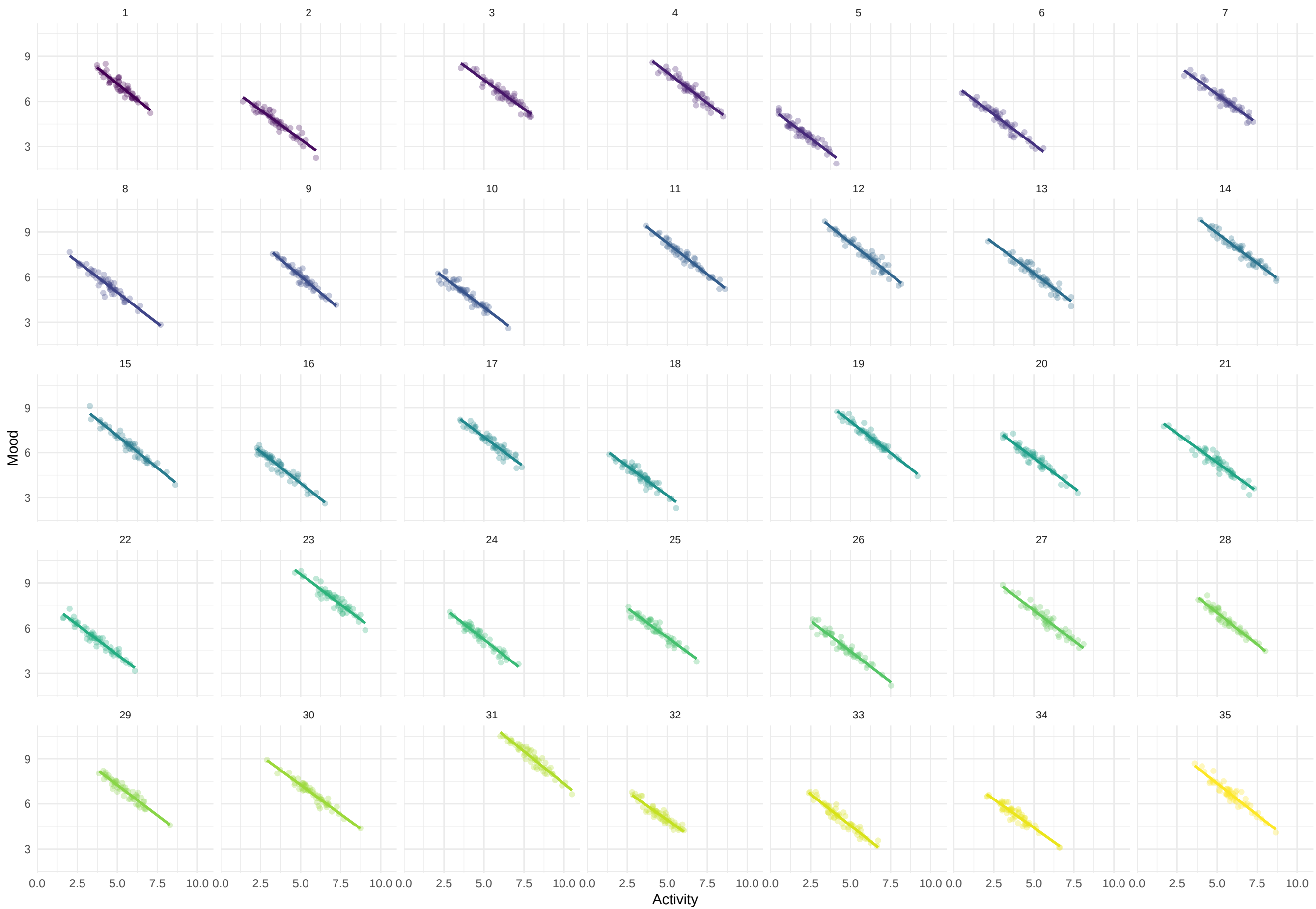
Individual Activity–Mood Relationships (35 people, 55 days each)
