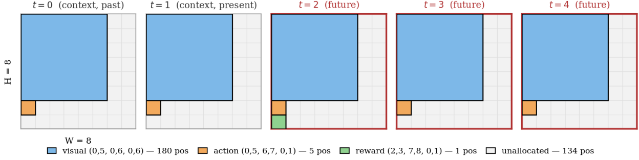
Figure 1: The exact layout declared by the code in §2.1, rendered as its five ( H, W ) time slices. visual occupies the 6 \times 6 block at every frame (180 positions), action one position per frame (5), and reward a single position at t = 2 . Frames t \geq t_{\text{current}} = 2 are future: denoised by reverse diffusion; earlier frames are clamped context. Unallocated positions (gray) carry no loss and no meaning.
