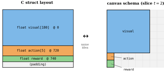
Figure 2: A C struct memory layout (left) and a canvas schema (right) are the same object: named fields at computed offsets, with a declared interpretation of every byte / position. The right panel is the t=2 slice of the layout in Fig. 1.
