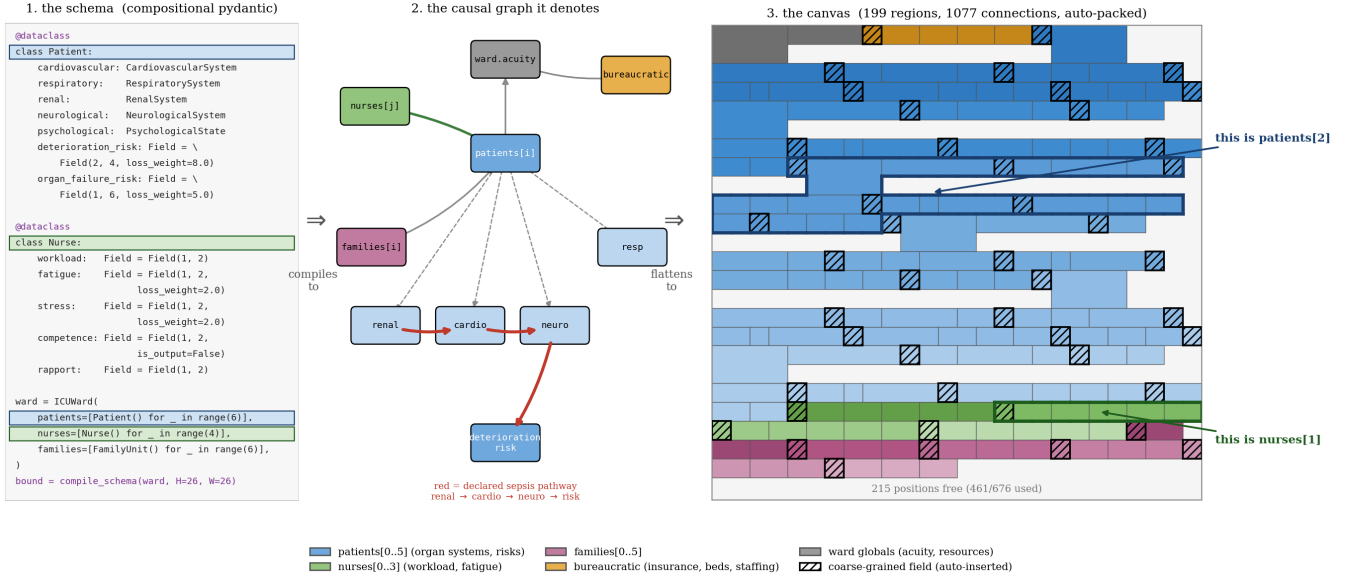
Figure 4: From schema to canvas, end to end, in three steps. 1: the declaration—Patient and Nurse types (abridged) and the ICUWard instance passed to the compiler. 2: the causal graph the schema denotes—composition and coordination edges, with the declared sepsis pathway (renal→cardio→neuro→deterioration_risk) highlighted. 3: the compiler’s output—199 typed regions and 1,077 connections auto-packed onto a 26 × 26 canvas (68% utilization). Nobody placed a rectangle by hand. Hatched blocks are the coarse-grained fields the compiler inserts at every nesting level; all cross-entity attention is forced through them, so the hierarchy of the schema becomes a hierarchy of bottlenecks on the canvas. Because the schema fixes what every position means, the latent tensor is pointable : the outlined runs of blocks are, exactly, patients[2] and nurses[1].
