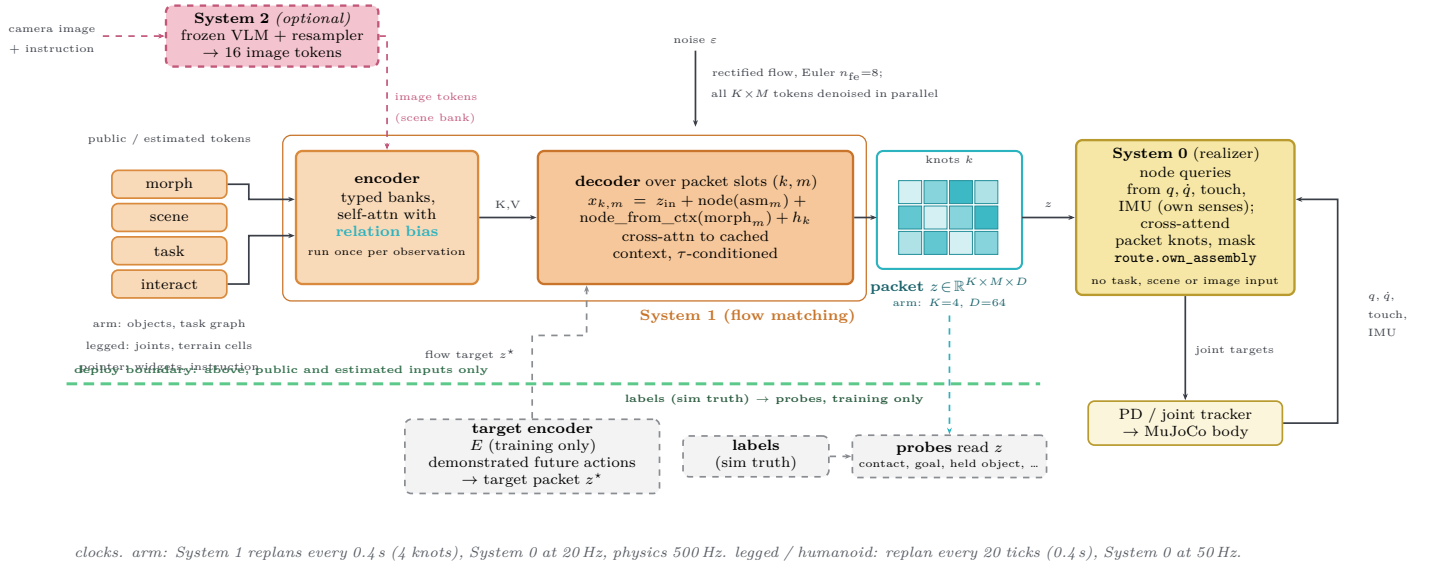
Figure 1: System overview. System 1 encodes typed context tokens (public or estimated fields only) once per observation and denoises the packet z in parallel; System 0 realizes the same z from the body’s own senses with no task, scene or image input. Dashed boxes are optional (System 2) or training-only (target encoder, labels, probes: simulator truth, never a deployed input).
