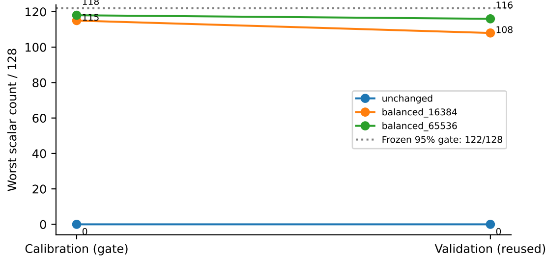
Original-mixture reused-validation minimum
