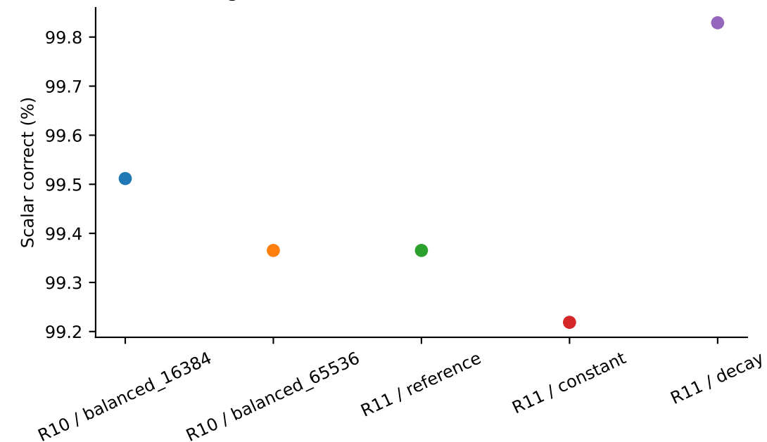
Original-mixture reused-validation minimum
