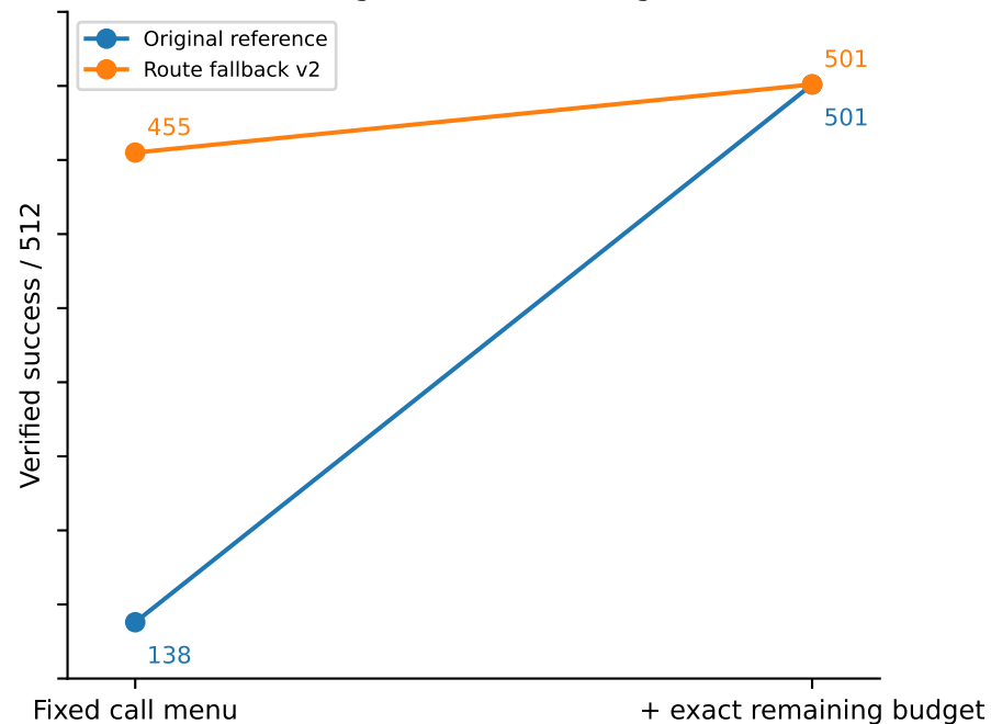
E02 tight 128-work budget
