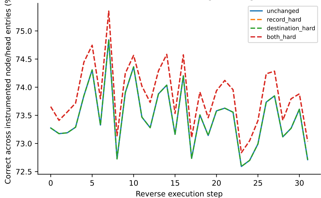
128 / 32: destination-head argmax diagnostic
