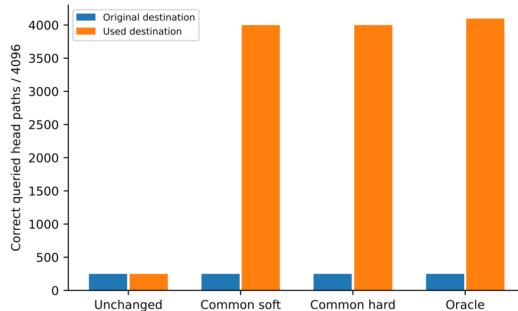
Deep query: individual-head full-route correctness
