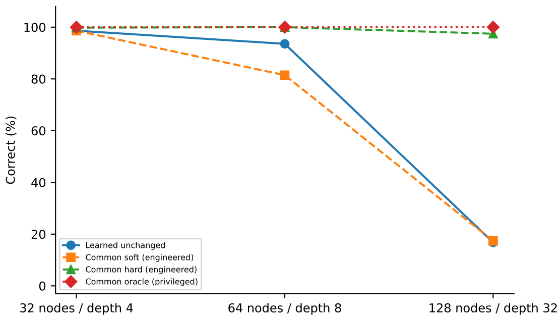
Task conditional on correct full query route
