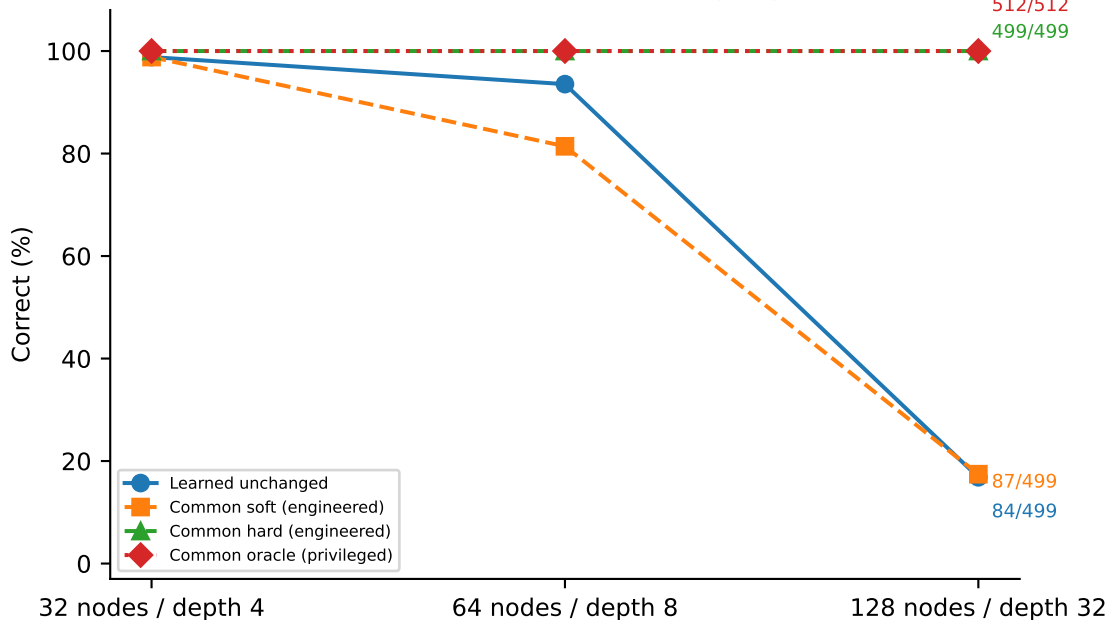
Task conditional on correct full query route
