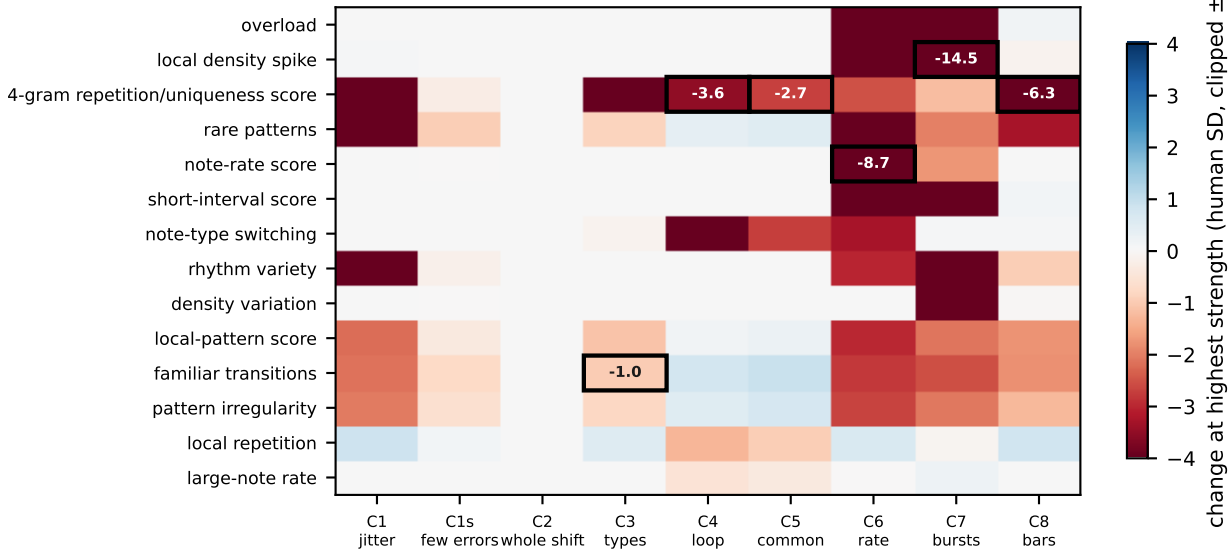
Calibrated chart-only scores under controlled damage black outline = frozen target; red = score falls, blue = rises
