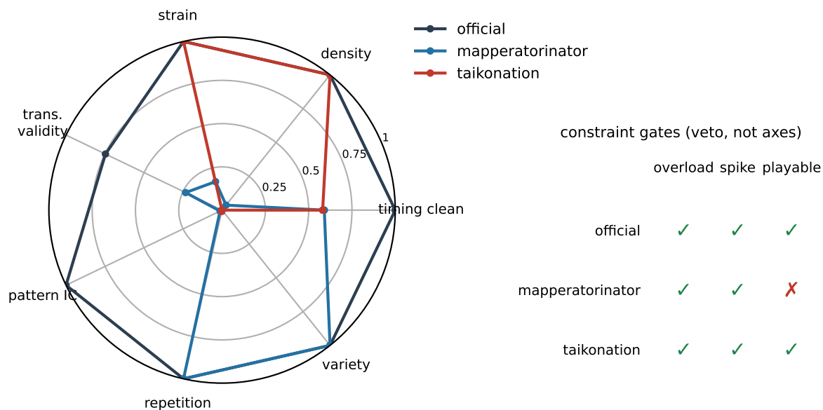
Figure 4: Ranker-axis profiles of the three taiko-vocabulary systems (radar; axes are 0–1 scores: timing clean rate and calibrated band scores; outline only—enclosed area is not a score). The two generated systems deviate on complementary axes: TaikoNation (red) holds density and strain but collapses on every pattern axis; Mapperatorinator (blue) holds repetition and variety but collapses on density and strain. Right: constraint gates, reported separately because gates veto rather than average (pass = median band score \geq 0.5 ); Mapperatorinator trips the playability gate. Cross-vocabulary systems appear in Figure 3 and the text: their time-based quantities are computable but read against taiko course norms, and their token-based families do not apply. The official row reads 0.75 on transition validity because a fixed training-corpus LM assigns nonzero unseen-transition rates to new songs; that value, not 1.0, is the human reference level for that axis.
