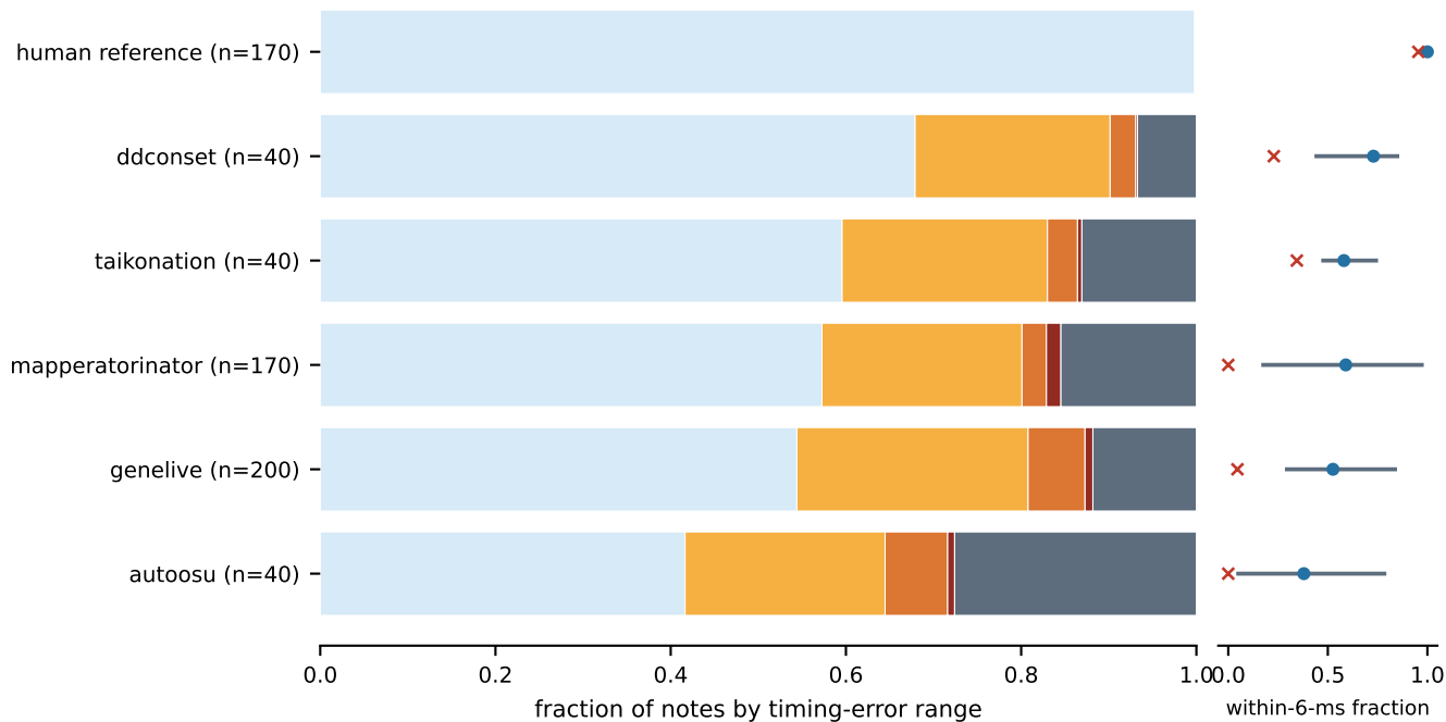
timing of evaluated systems (development songs, metadata-based grid)
