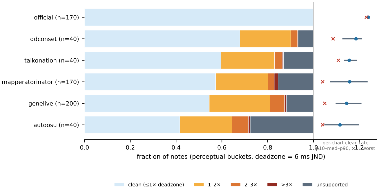
timing profiles of published systems (held-out test songs, authored grid)
