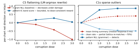
Figure 1: Two corruptions that one metric family does not register and another detects, as per-chart net direction (fraction of charts moving up minus moving down relative to their own intact version; null width \approx \pm 0.15 ). Left (C5 flattening) : rewriting notes toward the LM argmax drives n -gram NLL down in every chart (net direction −1.0 at full dose)—an improvement under the standard lower-is-better reading—while the band score built on the same LM statistic shows no dose-consistent reward (net direction +0.18/+0.28/+0.04 across doses): it is bounded at typicality. Right (C1s sparse outliers) : displacing 0.5–2% of notes by \pm 60 ms leaves mean timing summaries with zero median response (their dashed net-direction curve reflects sub-resolution drift with no usable magnitude), moves the timing clean rate in 34–45% of charts (the subdivision lattice re-matches \approx 70\% of displaced notes within the dead-zone), but flips the IOI token class of adjacent intervals, so grammar NLL responds with net direction +0.77 at one to three displaced notes per chart, rising to +0.87 at higher doses. Timing damage that placement metrics absorb is detected as grammar damage.
