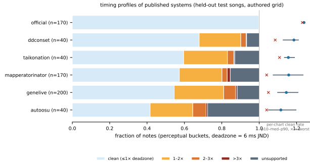
Figure 3: Timing profiles of published systems on the held-out test set (authored grid). Bars show the mean over charts of per-chart bucket fractions—clean ( \leq 1\times the 6 ms deadzone), tier exceedances, and unmatched—with rows ordered by the same statistic; n is the number of charts (difficulty-conditioned systems produce one chart per official course, others one per song). Right strip: per-chart clean-rate p10–median–p90 with the worst chart marked \times —tail charts that corpus means hide. The official row is all-clean by construction (officials are authored on the grid that defines cleanliness) and serves as a consistency check.
