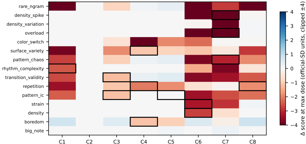
Metric coupling under targeted corruption (black boxes = designated targets)
