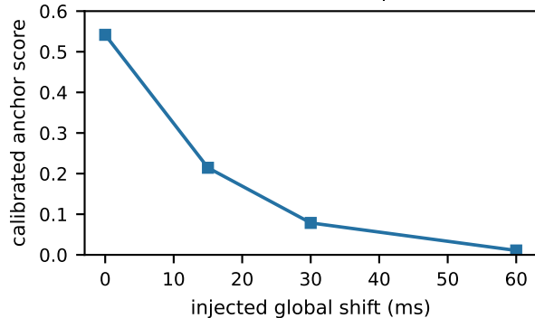
calibrated score response
