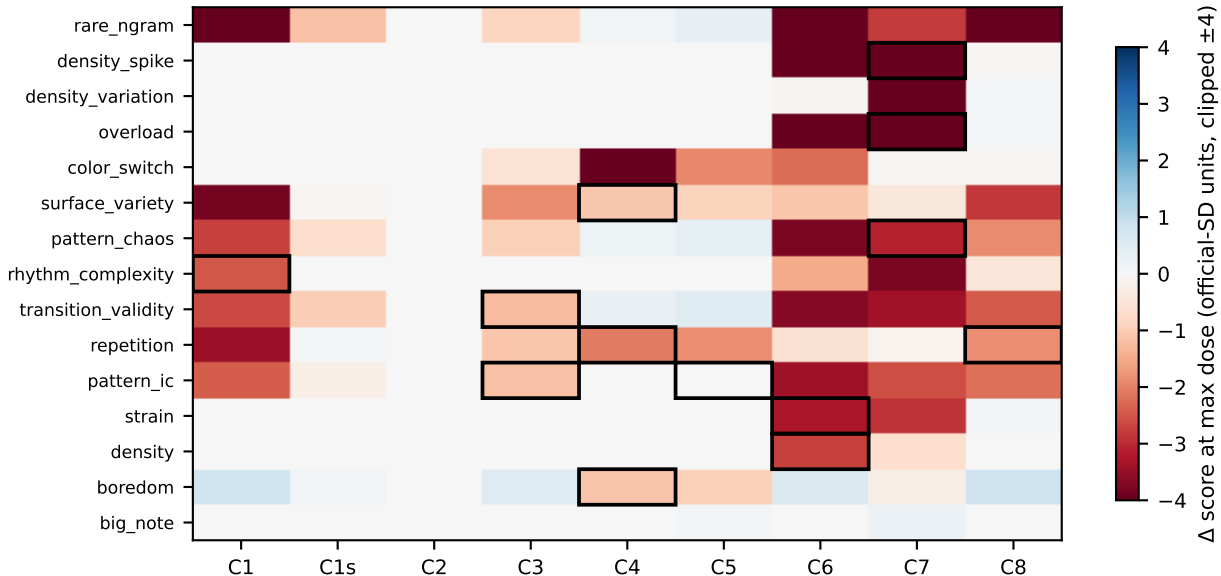
Metric coupling under targeted corruption (boxes = designated targets; C1s: discovered coupling)
