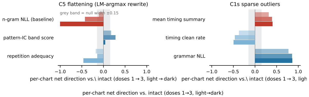
Figure 1: Two corruptions that one metric family does not register and another detects. Bars show per-chart net direction (fraction of charts moving up minus moving down relative to their own intact version) at doses 1–3, shaded light to dark; the grey band is the null width \approx \pm 0.15 . Left (C5 flattening): rewriting notes toward the LM argmax drives n -gram NLL down in every chart ( -1.0 at full dose)—an improvement under the lower-is-better reading—while the band score over the same statistic shows no dose-consistent reward ( +0.18/+0.28/+0.04 , bounded at typicality) and repetition adequacy registers the induced looping. Right (C1s sparse outliers): displacing 0.5\text{--}2\% of notes by \pm 60 ms leaves mean timing summaries with zero median response (their positive net direction reflects sub-resolution drift with no usable magnitude), moves the timing clean rate in 34\text{--}45\% of charts (the subdivision lattice re-matches \approx 70\% of displaced notes within the deadzone), but flips the IOI token class of adjacent intervals: grammar NLL responds at +0.77 with one to three displaced notes per chart, rising to +0.87 .
