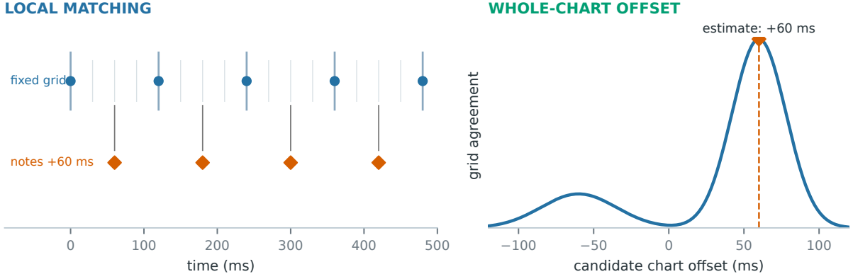
Figure 3: Why timing needs a whole-chart estimate. Left: nearest-grid matching can pair shifted notes with different subdivision points and report small local errors. Right: a schematic agreement curve over candidate whole-chart offsets; its maximum recovers the injected +60 ms shift. The grids are fixed before evaluating the generated chart.
