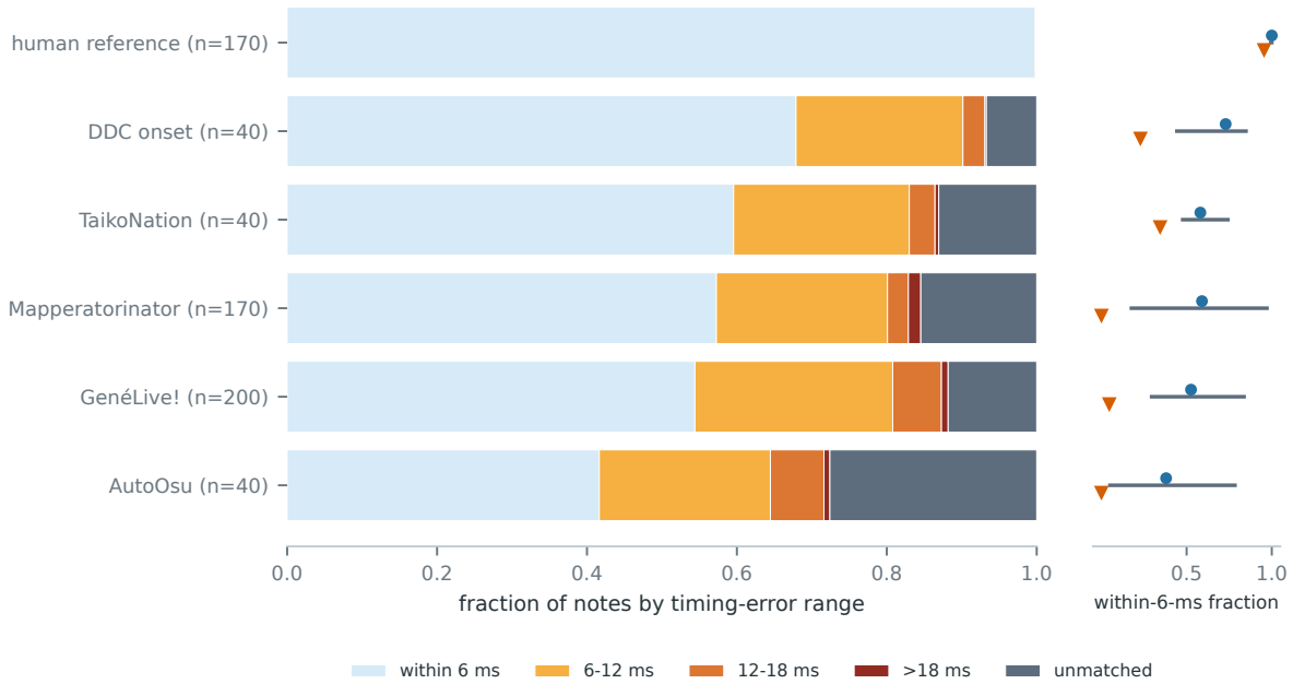
Figure 5: Timing of the evaluated systems on the 40 development songs using the authored grid. Each bar is the mean fraction of notes within 6 ms and in the 6–12, 12–18, and above-18 ms ranges, or unmatched; n is the number of charts. In the right strip, the horizontal line spans the 10th–90th percentiles, the dot marks the median, and a downward triangle marks the minimum within-6 ms fraction. Similar mean clean fractions can coexist with different timing tails.
