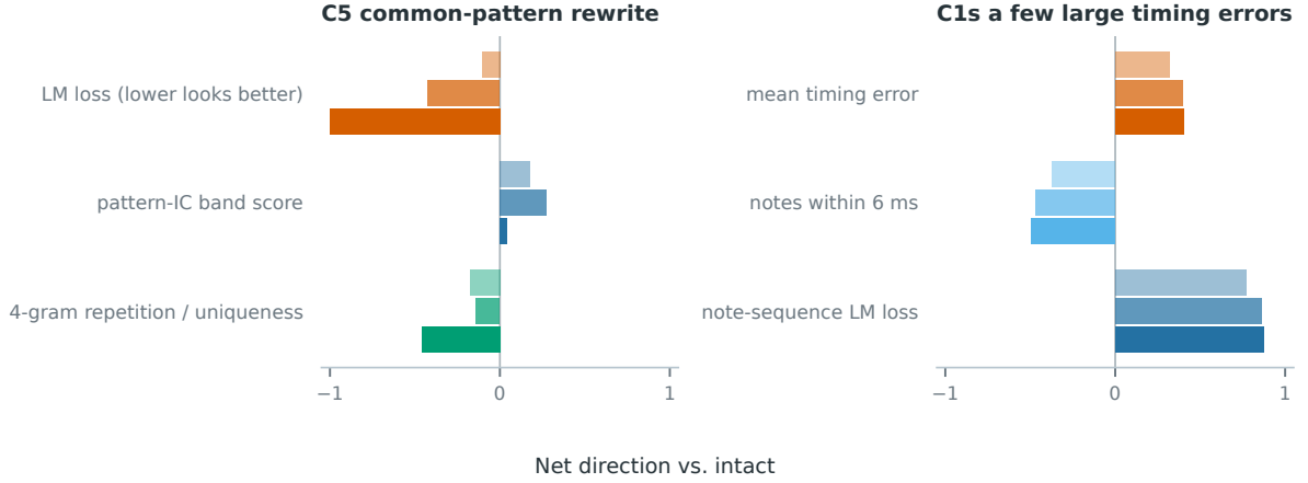
Figure 4: Two cases in which one measurement misses a targeted change and another responds. Bars show the fraction of charts moving up minus the fraction moving down relative to the intact chart; light to dark marks the three corruption strengths on the development panel (descriptive, not independent-chart confidence statements). Left: common-pattern rewriting lowers LM loss and raises the pattern-IC band score, while the 4-gram repetition/uniqueeness axis moves the other way (its two algebraically equivalent output names are plotted once). Right: sparse \pm 60 ms timing errors leave the mean timing error near zero and are mostly re-paired by the nearest grid, while the note-sequence LM responds to the changed intervals.
