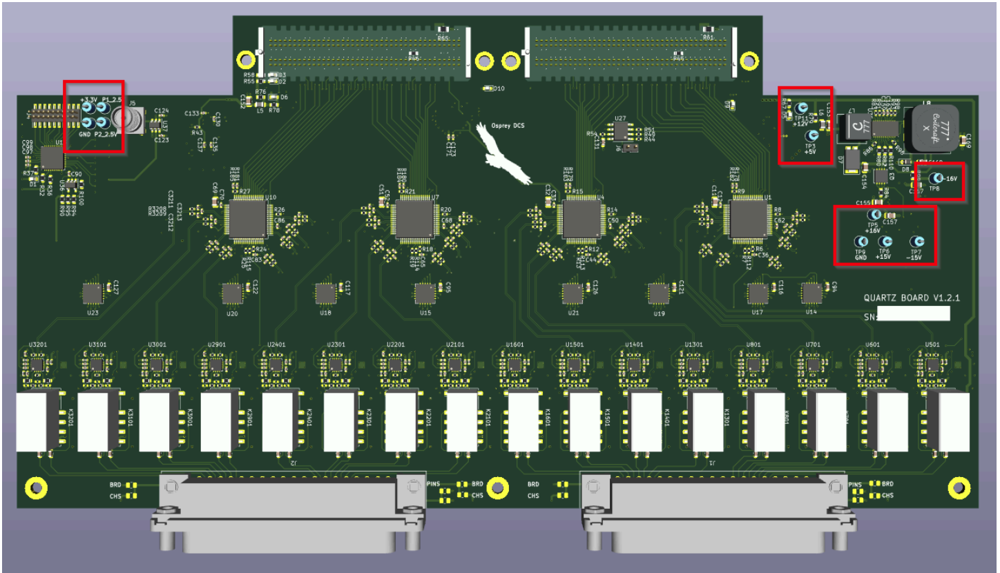
Image 1: 3D render of Quartz Boards with test points called out
