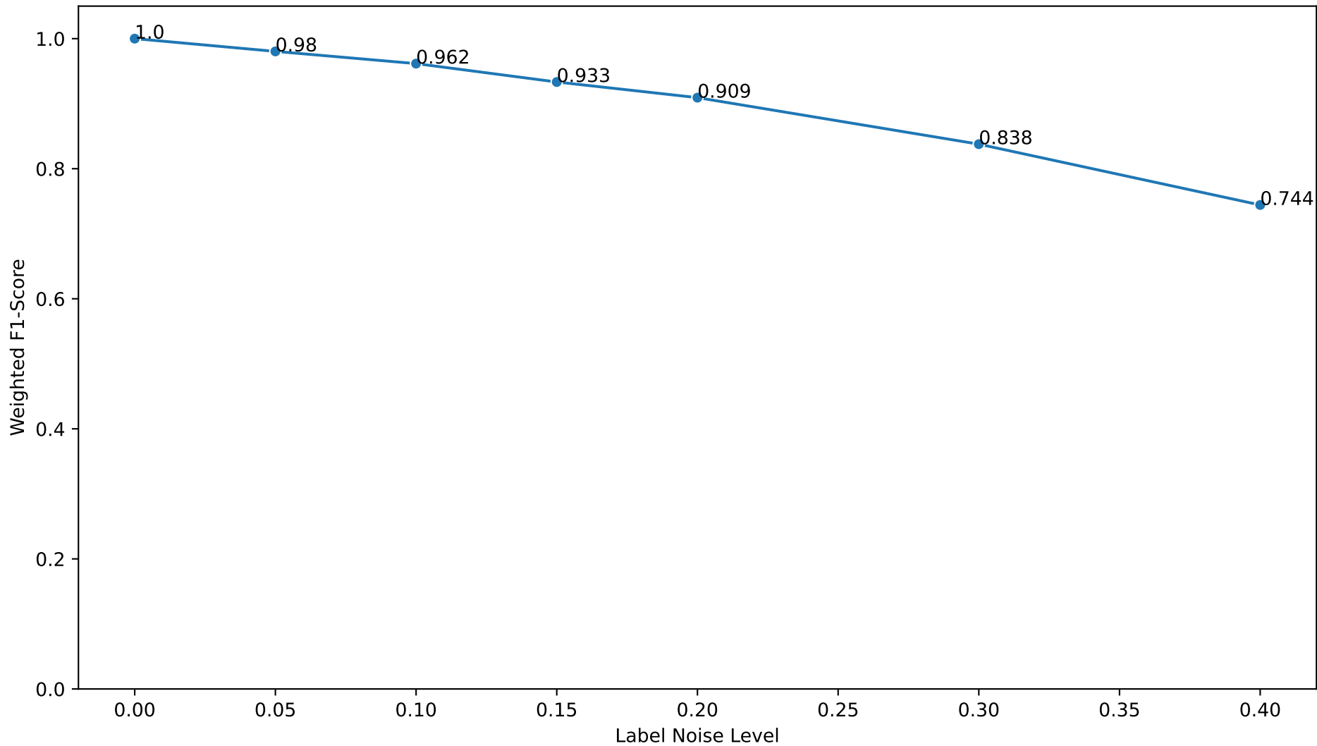
RQ6 Robustness Under Increasing Label Noise
